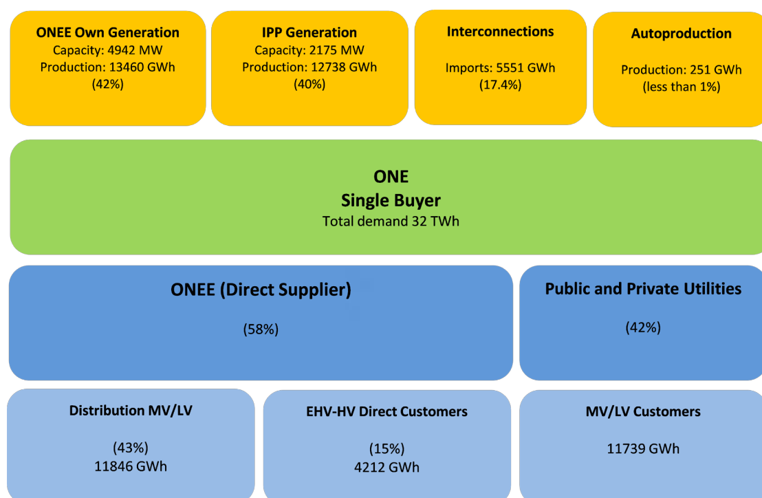
Figure 5 | Balance of supply-demand, 2012
